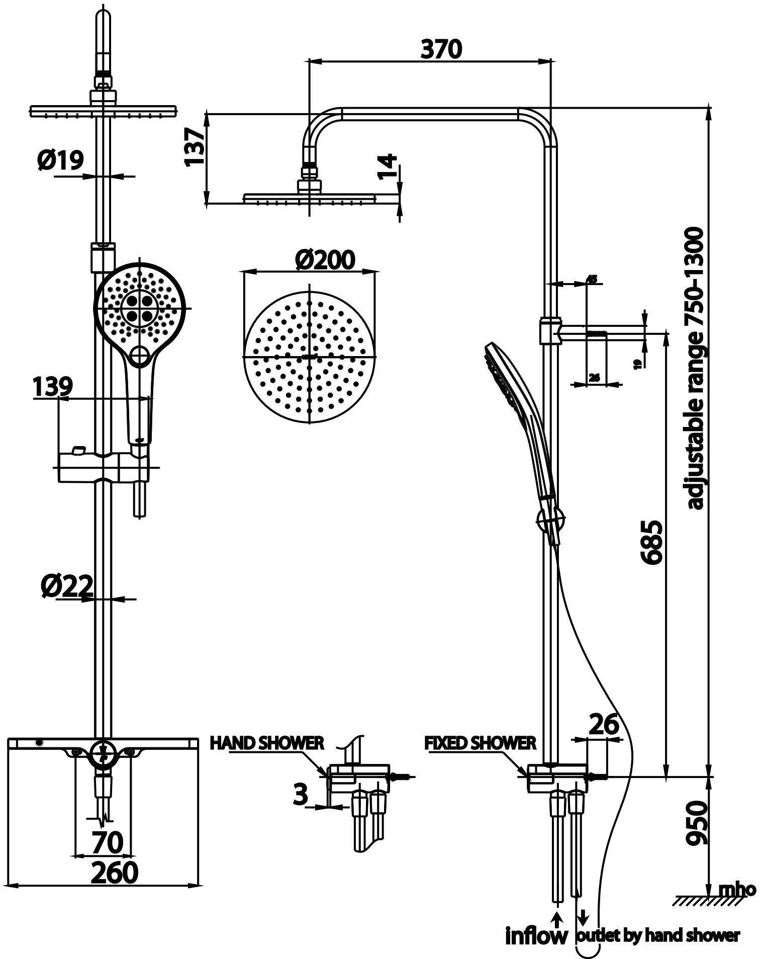
RAIN SHOWER SET WITH SAELF AND SWITCH BUTTONS
