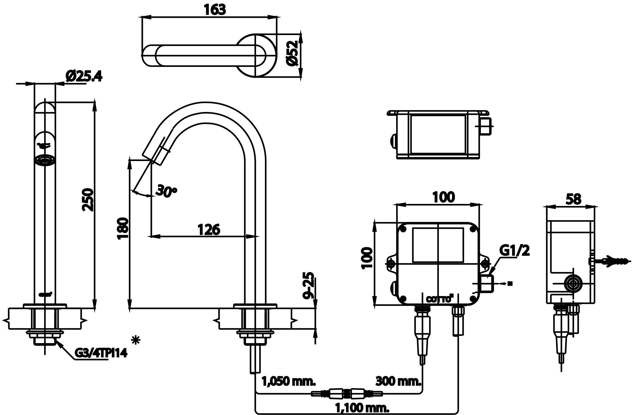
AUTOMATIC FAUCET CT4912DC
