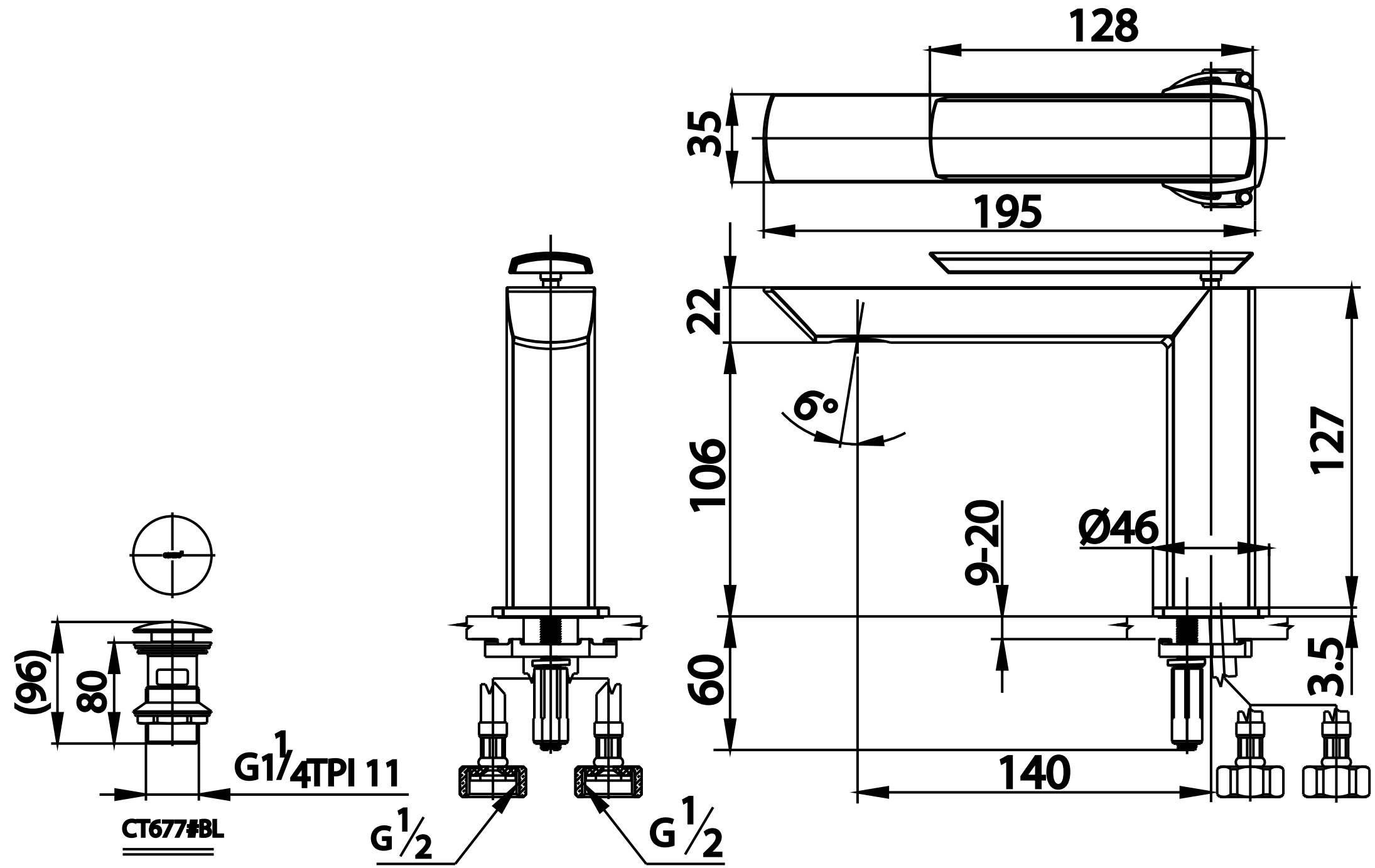
BASEN MIXER FAUCET WITH INLET HOUSE AND BLACK COLOR WASTE CT2281A#BL
