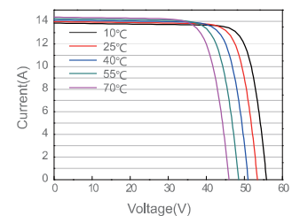
Current-Voltage Curve JAM78S30-595/MR
